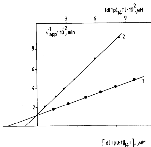
Fig. 1. Dependence of k_{app} of DNA polymerase inactivation in the reaction of DNA polymerization on the concentration of d(Tp)_{14}T (1) and d[ Tp(Et) ]_{14}T (2) at fixed concentration of d(pT)_2pC[Pt^{2+}(NH_3)_2OH](pT)_7 equal to 1 \mu M .
